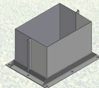
TRUNKING - Honeyville's unique design utilizes ten 90° bends for greater vertical strength and structural integrity.
