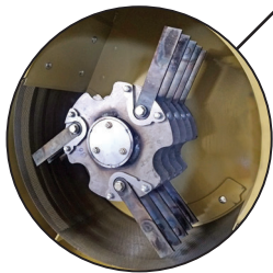
Improved Mill Design Featuring Restricted Hinge Hammers and Reinforced Screen Holder
