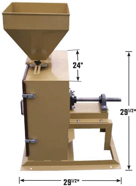
18" Mill Shown With Jackshaft Assembly, Intake Hopper & Slide
